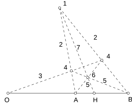
harmonic mean
